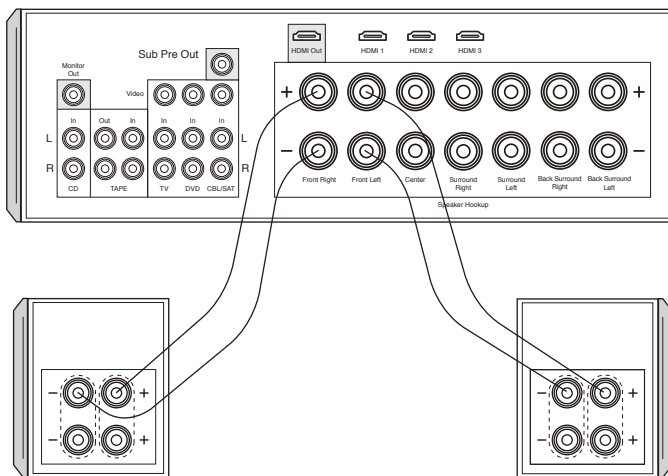
Figure 5 Raccordements standard
