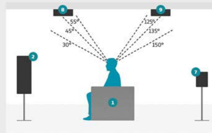
Overhead speaker placement detail for 9.1.4 setup
